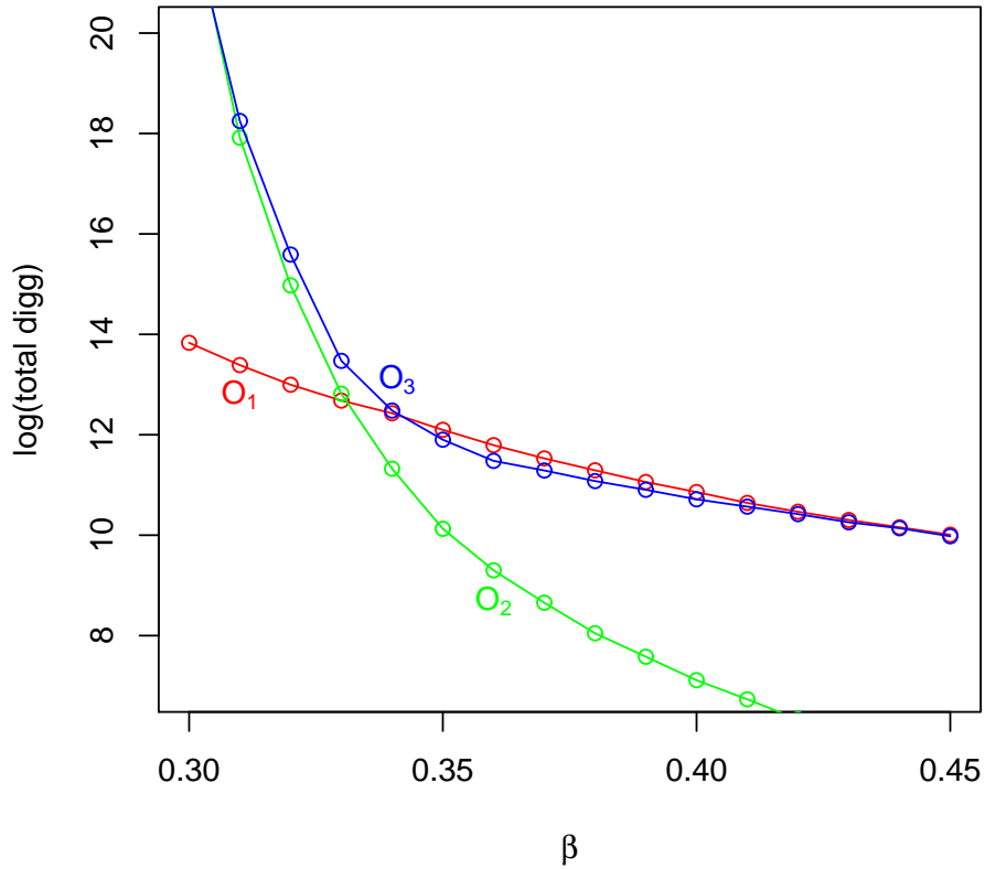
Figure 4 – The total number of diggs generated using three ordering strategies O_1 , O_2 , and O_3 , for \alpha = 0.4 and a range of \beta . The novelty factor decays as r_t = e^{-\alpha t^\beta} . Performance is measured by the logarithm of the total number of diggs generated in 10,000 time steps. As can be seen, O_3 asymptotically approaches O_1 and O_2 in the fast decay (large \beta ) and slow decay (small \beta ) limit, respectively. A phase transition happens around \beta = 0.335 .
